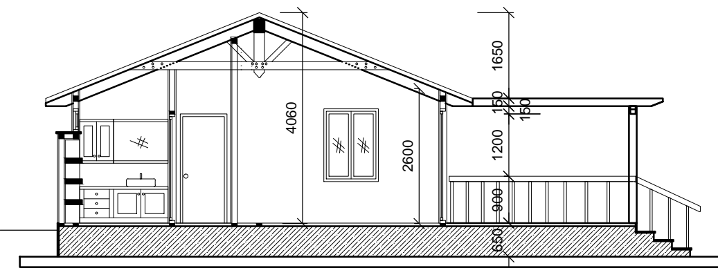
SNID B1-B1
