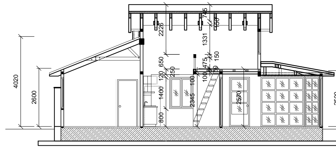
SNID B-B
